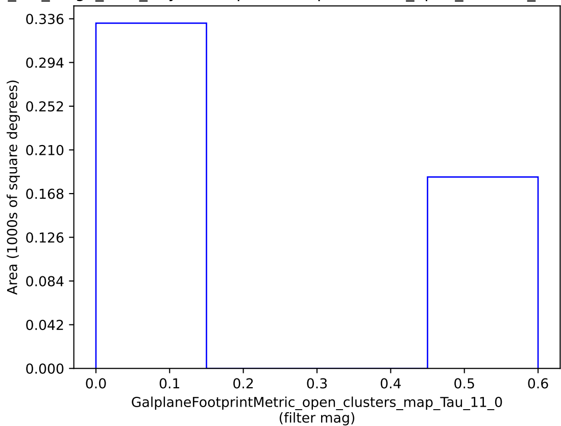
mw_roll_bulge_v3.3_10yrs : GalplaneFootprintMetric_open_clusters_map_Tau_11_0
