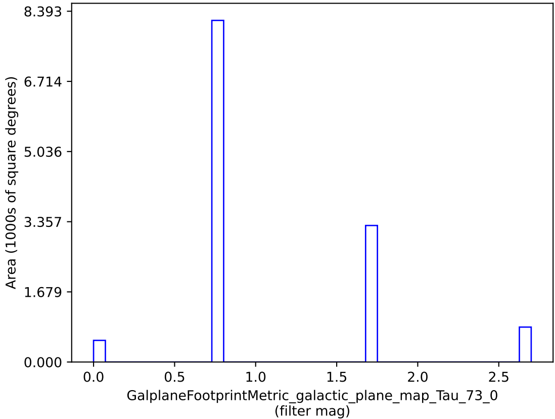
mw_roll_bulge_v3.3_10yrs : GalplaneFootprintMetric_galactic_plane_map_Tau_73_0
