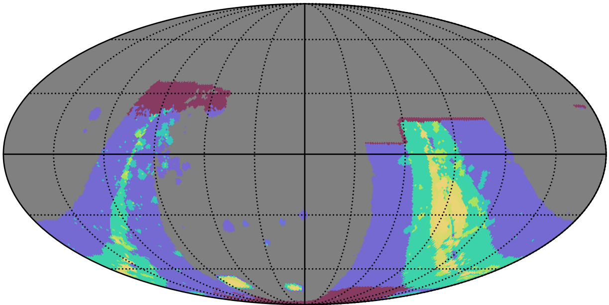
mw_roll_bulge_v3.3_10yrs : GalplaneFootprintMetric_combined_map_Tau_46_5
