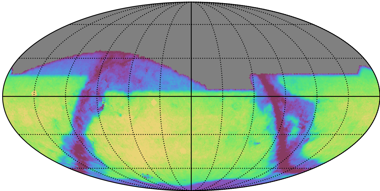
mw_roll_bulge_v3.3_10yrs z: GalaxyCountsMetricExtended
