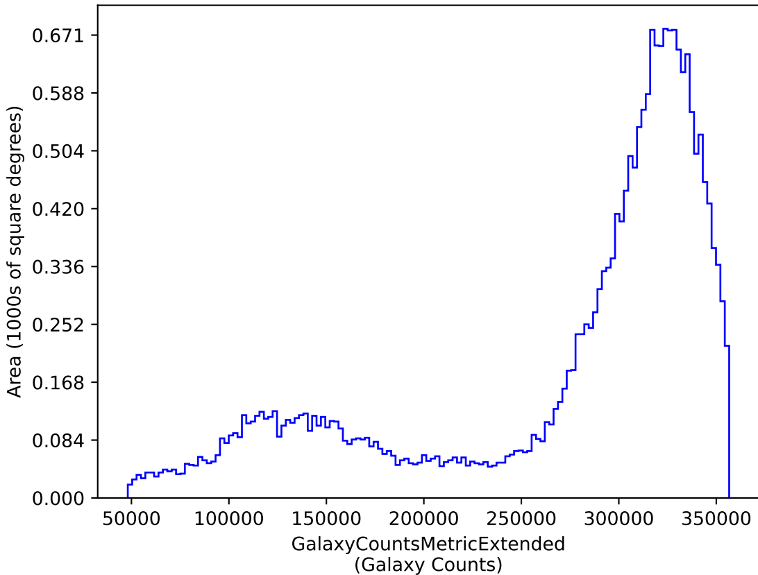
mw_roll_bulge_v3.3_10yrs y: GalaxyCountsMetricExtended
