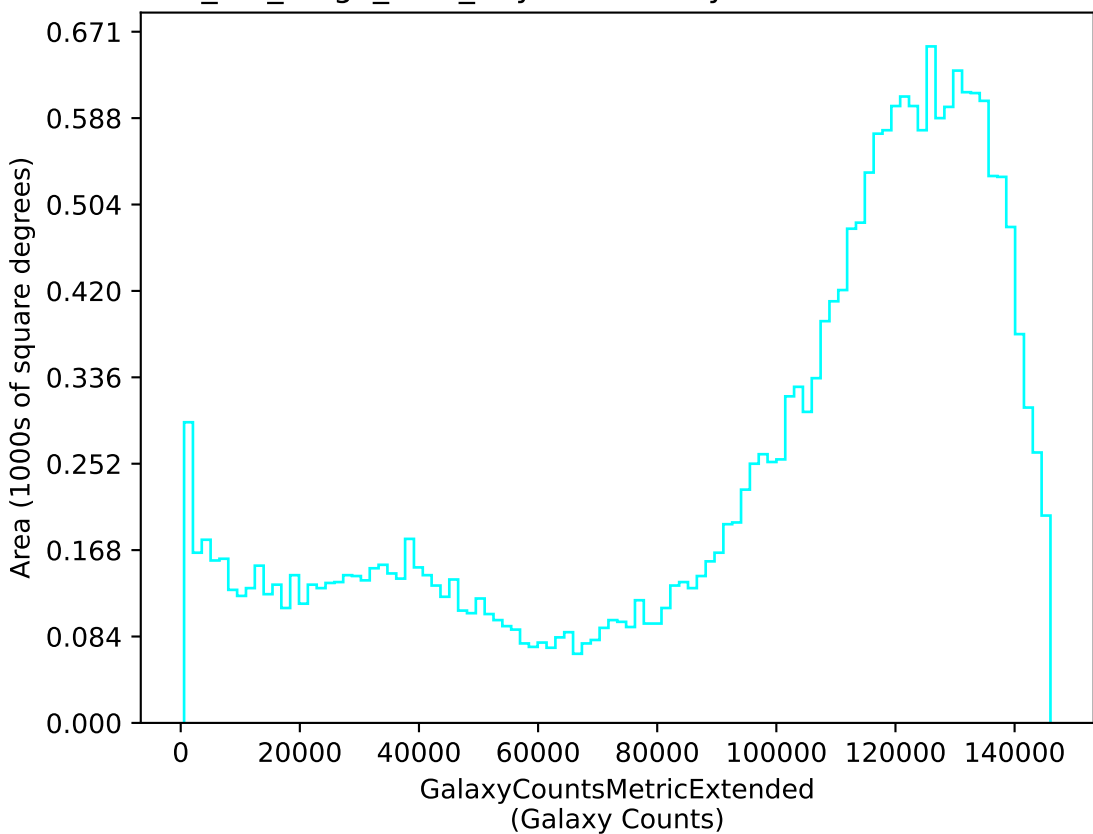
mw_roll_bulge_v3.3_10yrs u: GalaxyCountsMetricExtended
