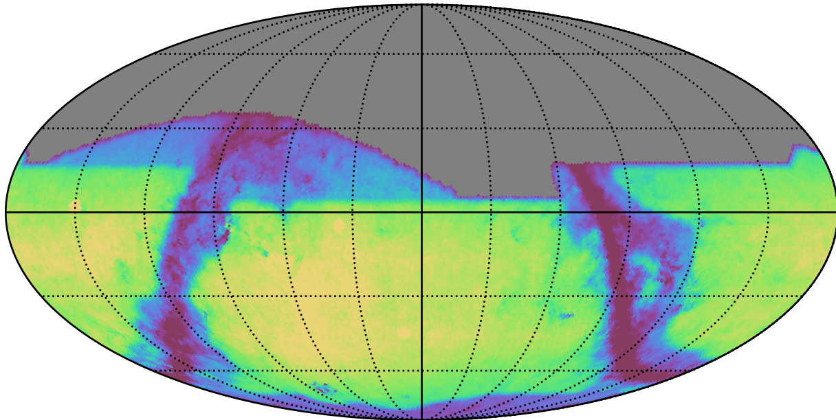
mw_roll_bulge_v3.3_10yrs i: GalaxyCountsMetricExtended
