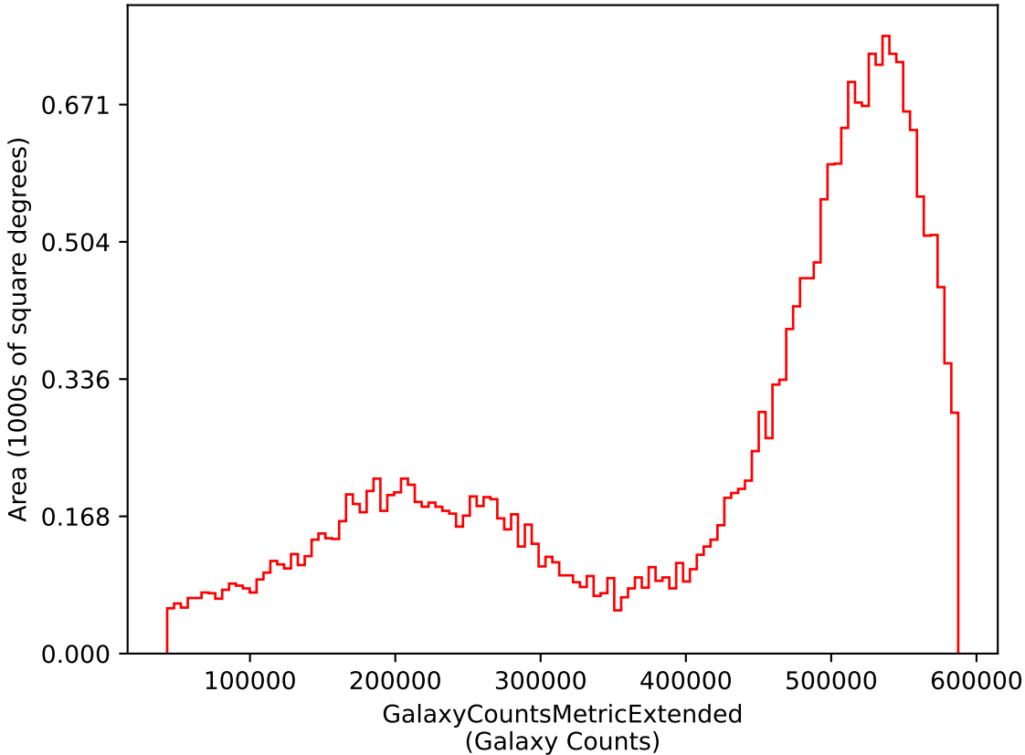
mw_roll_bulge_v3.3_10yrs i: GalaxyCountsMetricExtended
