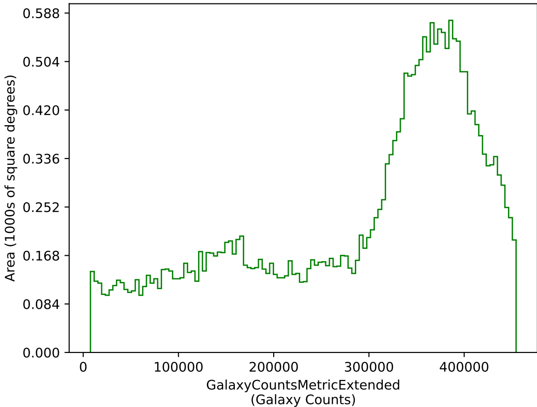
mw_roll_bulge_v3.3_10yrs g: GalaxyCountsMetricExtended
