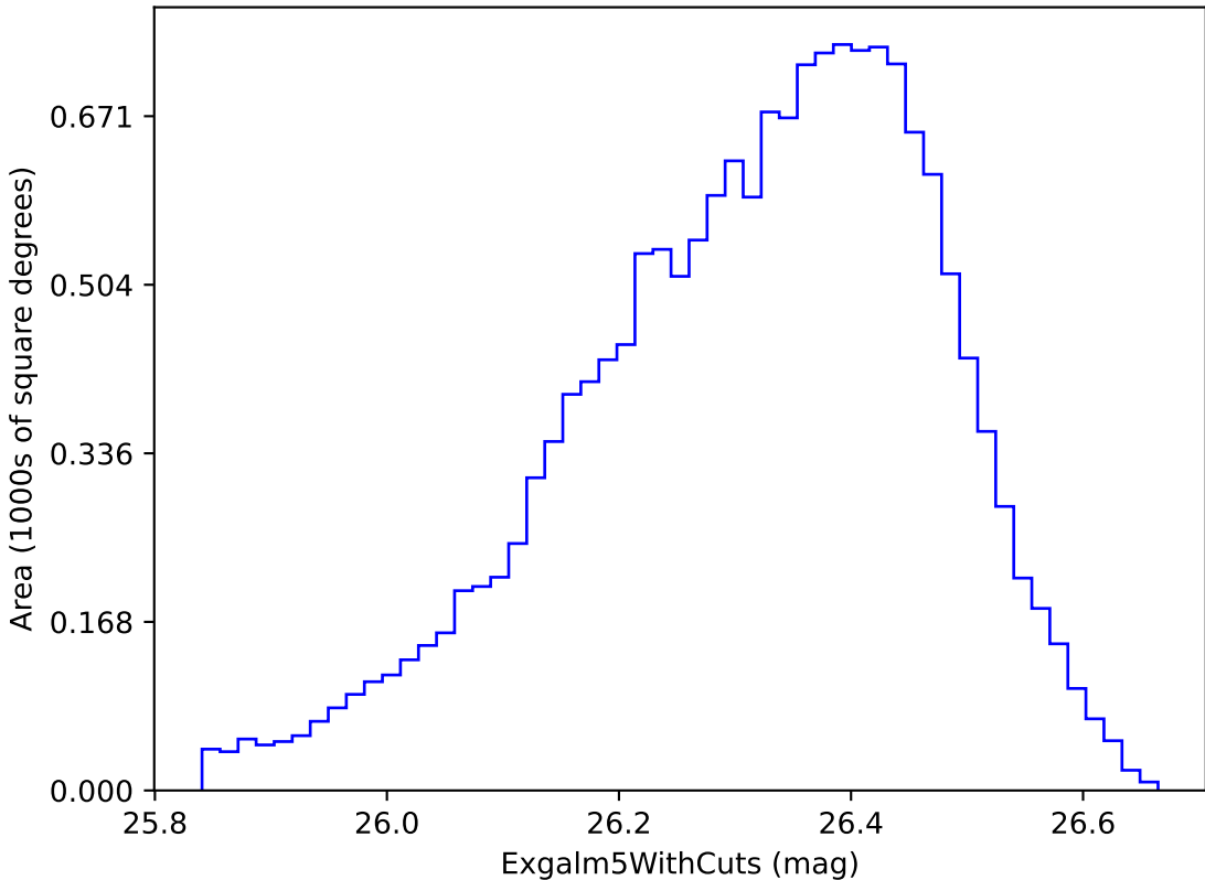
mw_roll_bulge_v3.3_10yrs i band non-DD year 9: ExgalM5WithCuts
