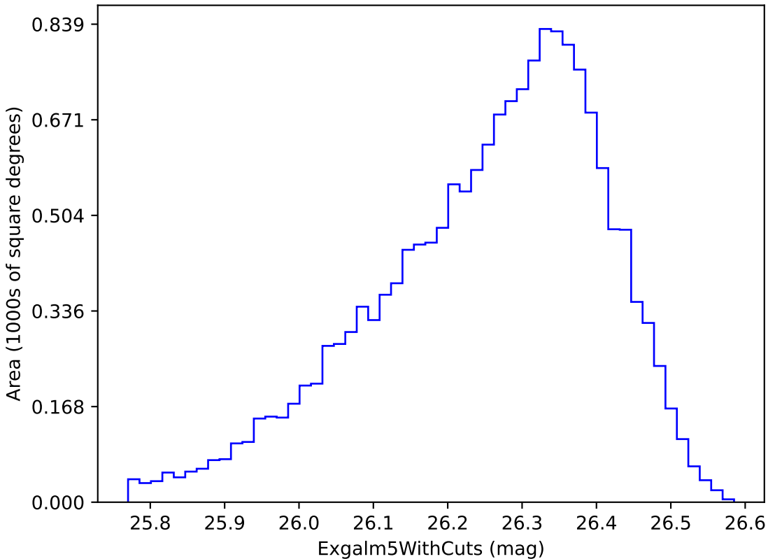
mw_roll_bulge_v3.3_10yrs i band non-DD year 8: ExgalM5WithCuts
