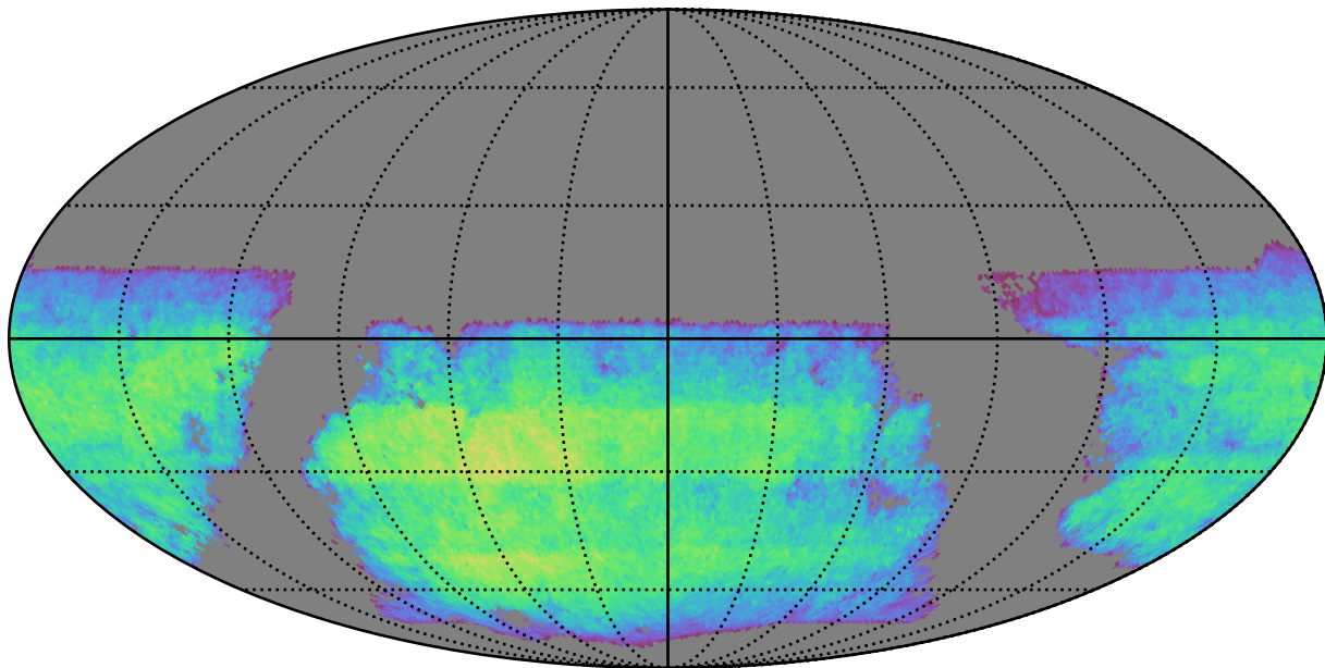
mw_roll_bulge_v3.3_10yrs i band non-DD year 7: ExgalM5WithCuts
