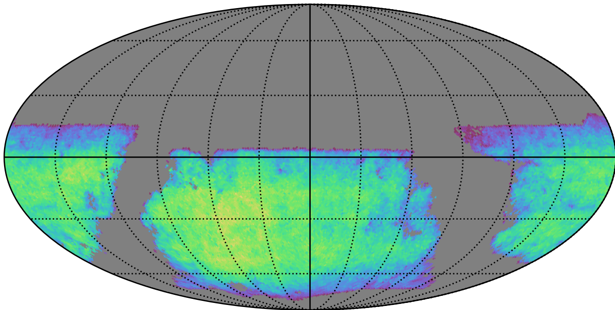
mw_roll_bulge_v3.3_10yrs i band non-DD year 6: ExgalM5WithCuts
