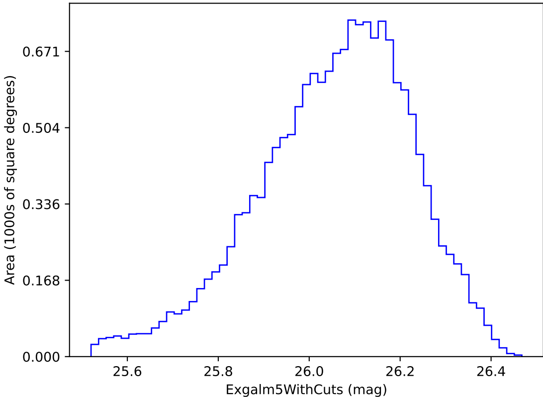
mw_roll_bulge_v3.3_10yrs i band non-DD year 5: ExgalM5WithCuts
