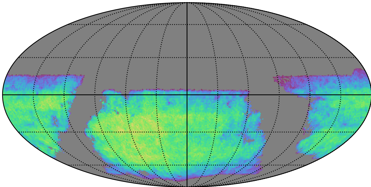
mw_roll_bulge_v3.3_10yrs i band non-DD year 4: Exgal5WithCuts
