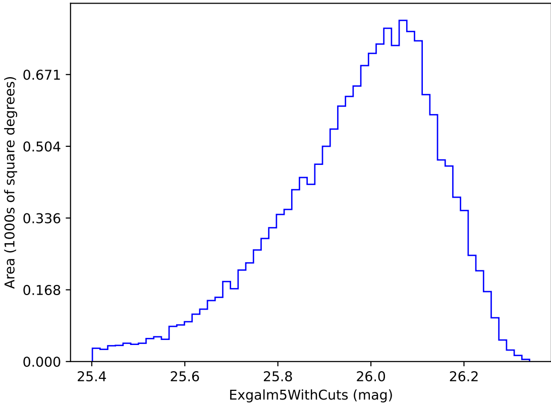
mw_roll_bulge_v3.3_10yrs i band non-DD year 4: Exgal5WithCuts
