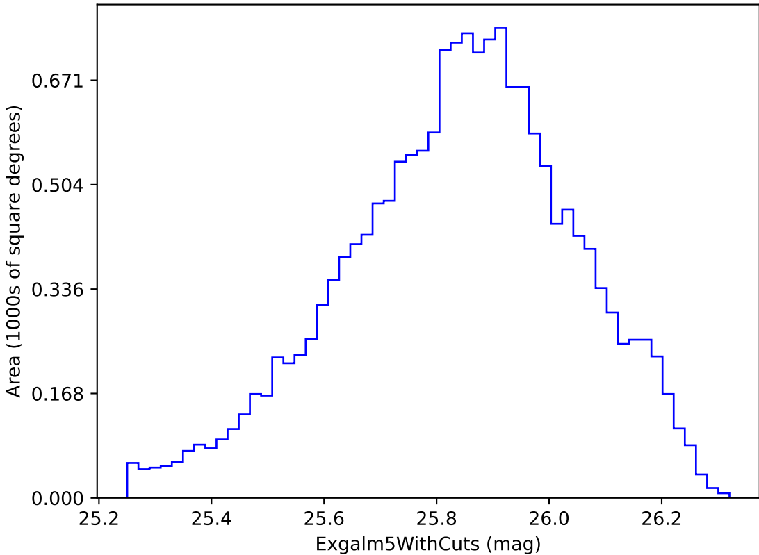
mw_roll_bulge_v3.3_10yrs i band non-DD year 3: ExgalM5WithCuts
