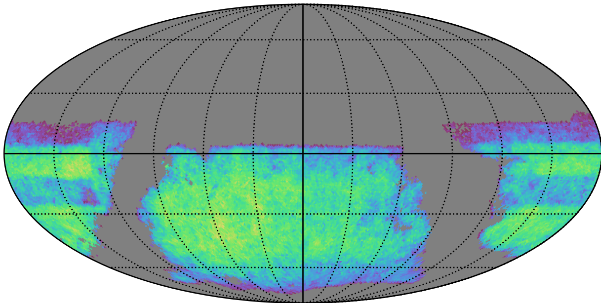
mw_roll_bulge_v3.3_10yrs i band non-DD year 2: ExgalM5WithCuts
