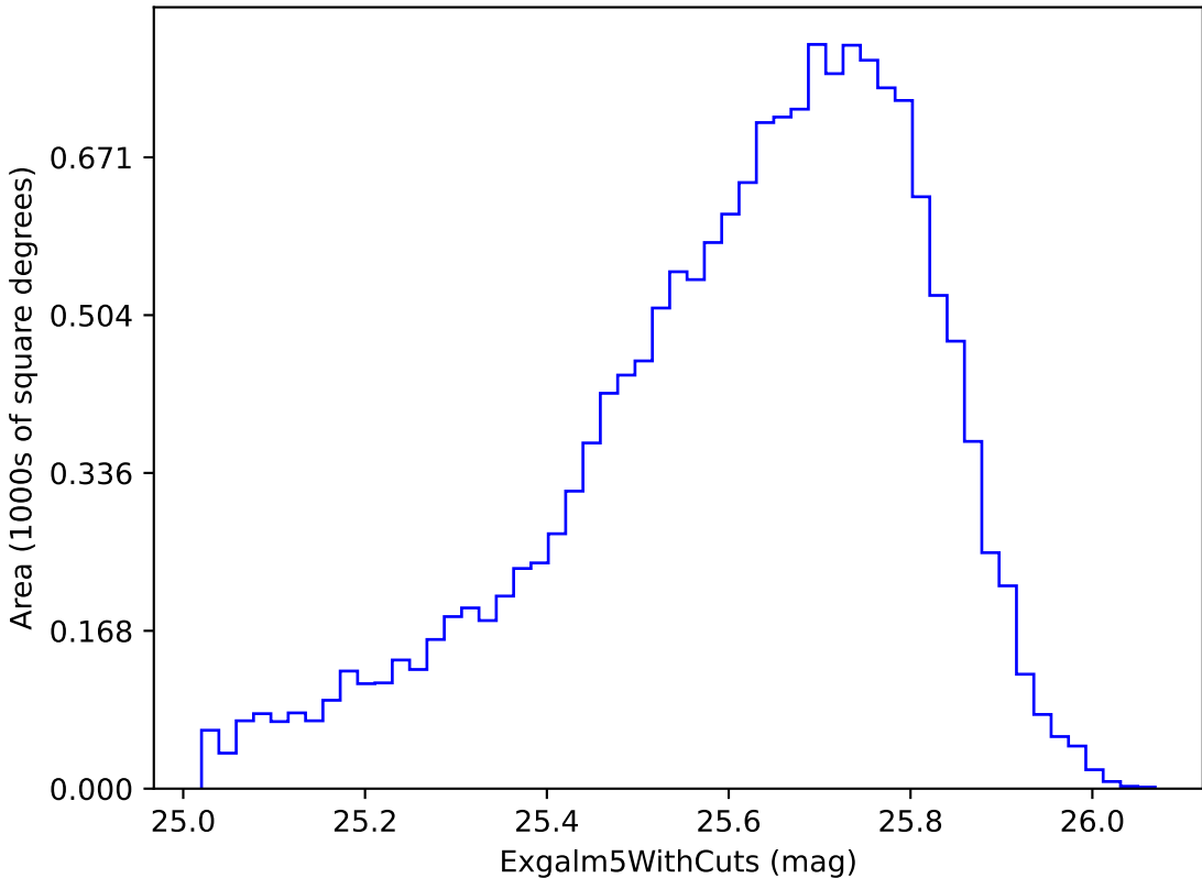
mw_roll_bulge_v3.3_10yrs i band non-DD year 2: Exgal5WithCuts
