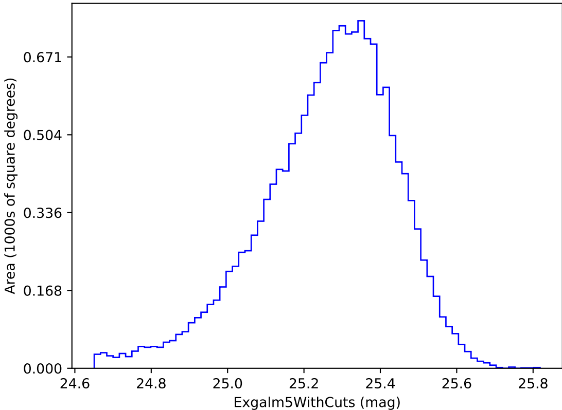
mw_roll_bulge_v3.3_10yrs i band non-DD year 1: ExgalM5WithCuts
