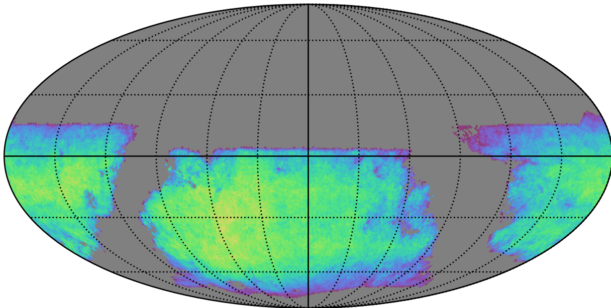
mw_roll_bulge_v3.3_10yrs i band non-DD year 10: Exgal m5 WithCuts
