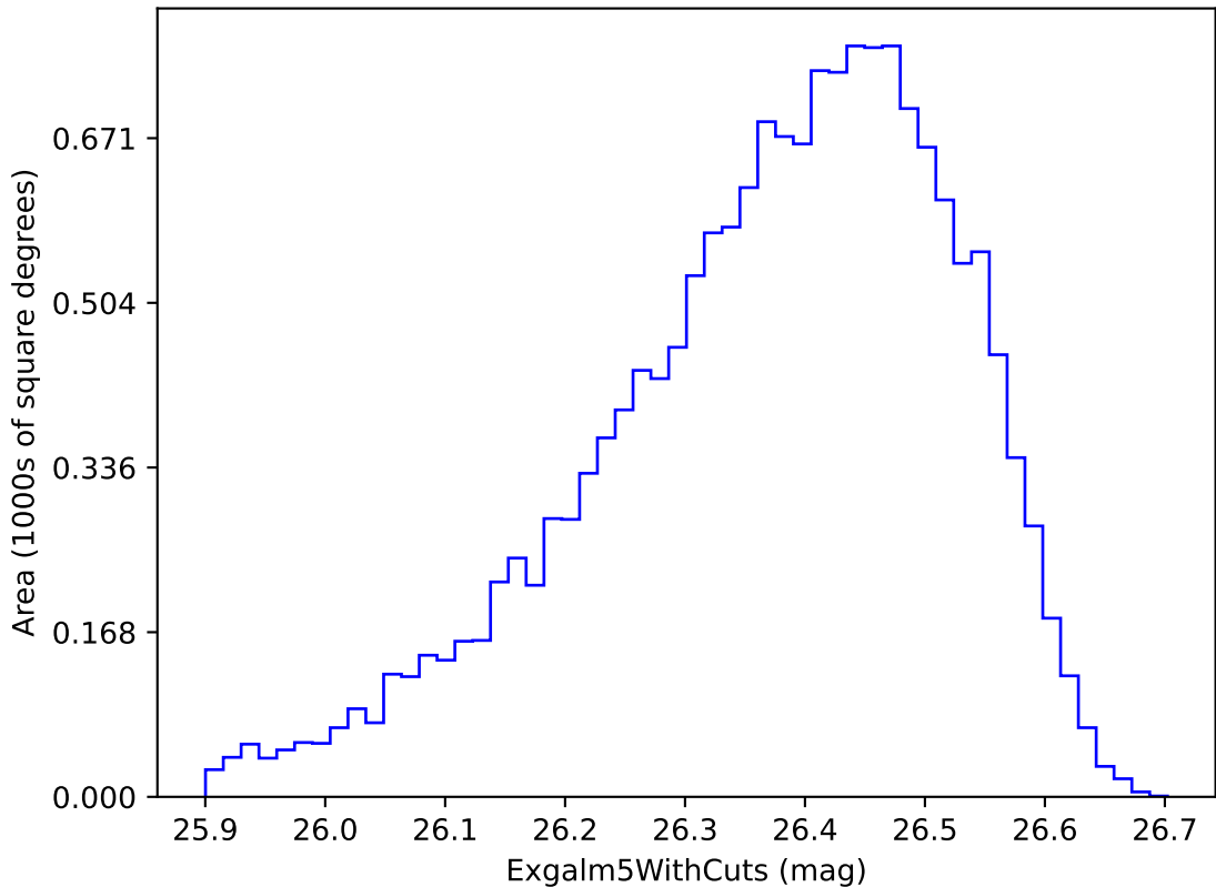
mw_roll_bulge_v3.3_10yrs i band non-DD year 10: ExgalM5WithCuts
