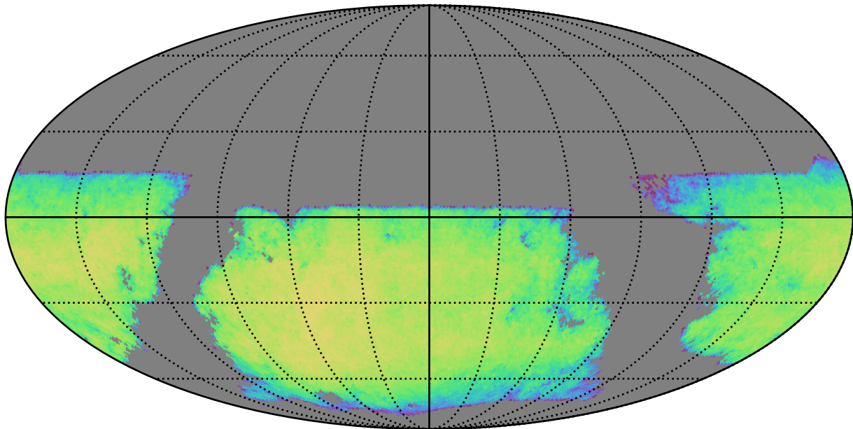
mw_roll_bulge_v3.3_10yrs i band galaxies non-DD: DepthLimitedNumGalaxiesMetric
