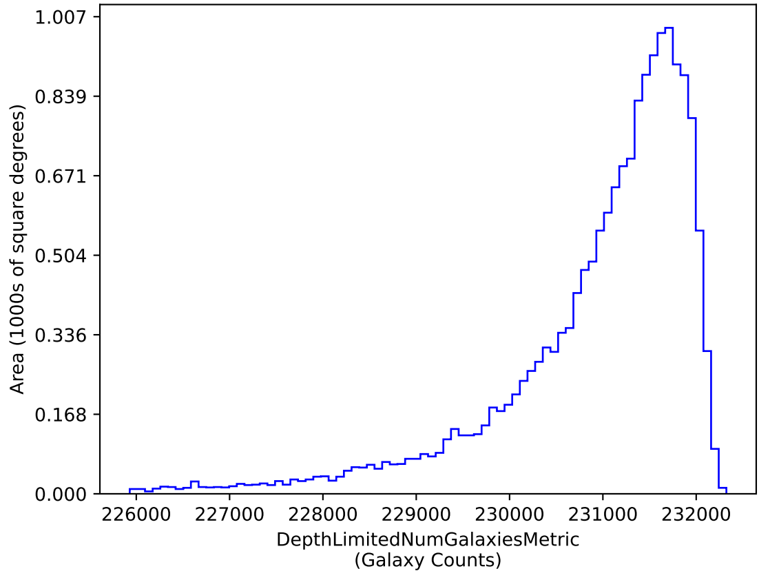
mw_roll_bulge_v3.3_10yrs i band galaxies non-DD: DepthLimitedNumGalaxiesMetric
