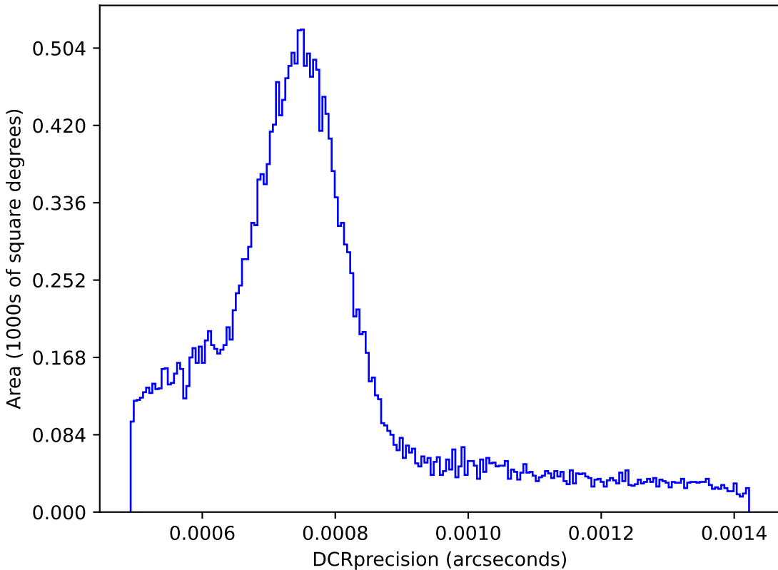
mw_roll_bulge_v3.3_10yrs : DCRprecision
