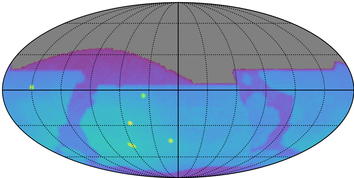
mw_roll_bulge_v3.3_10yrs : Brown Dwarf, L7
