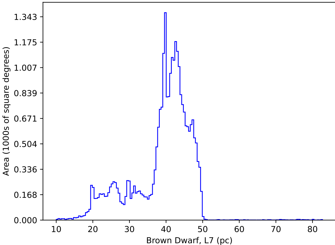
mw_roll_bulge_v3.3_10yrs : Brown Dwarf, L7
