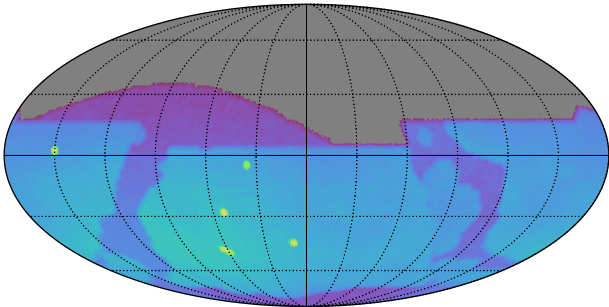
mw_roll_bulge_v3.3_10yrs : Brown Dwarf, L4
