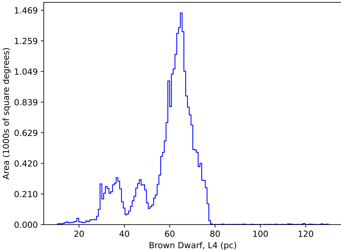
mw_roll_bulge_v3.3_10yrs : Brown Dwarf, L4
