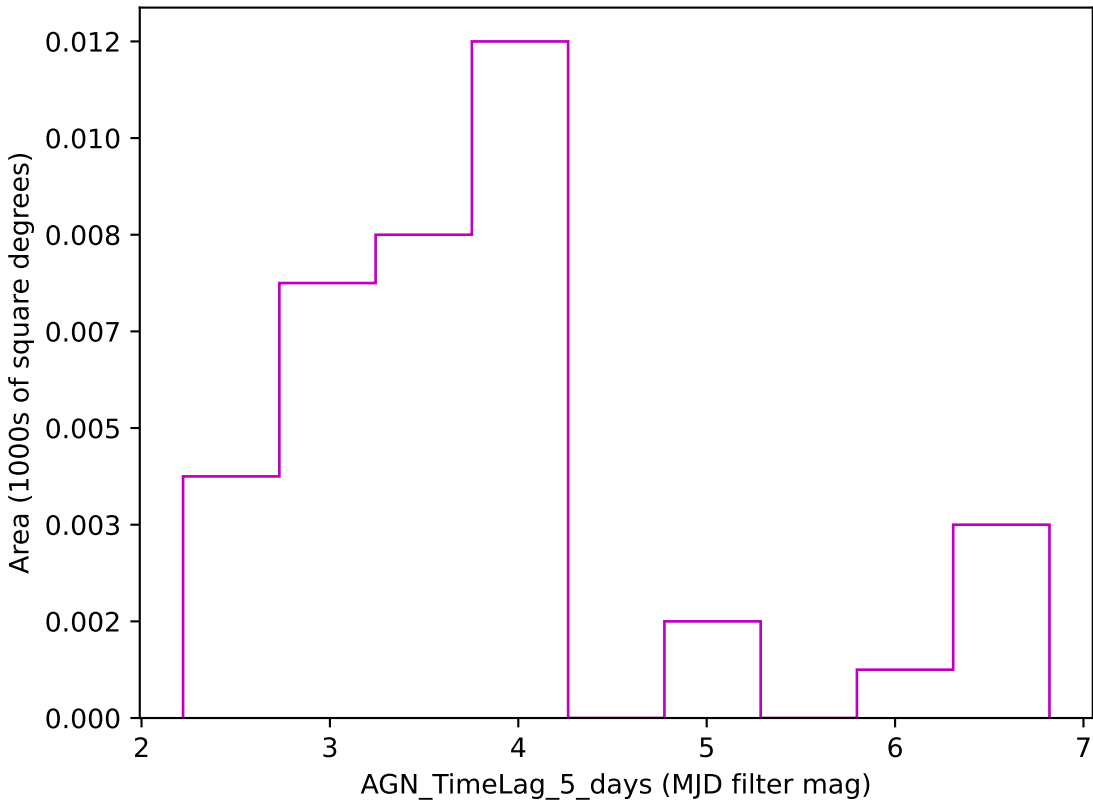
mw_roll_bulge_v3.3_10yrs z band: AGN_TimeLag_5_days
