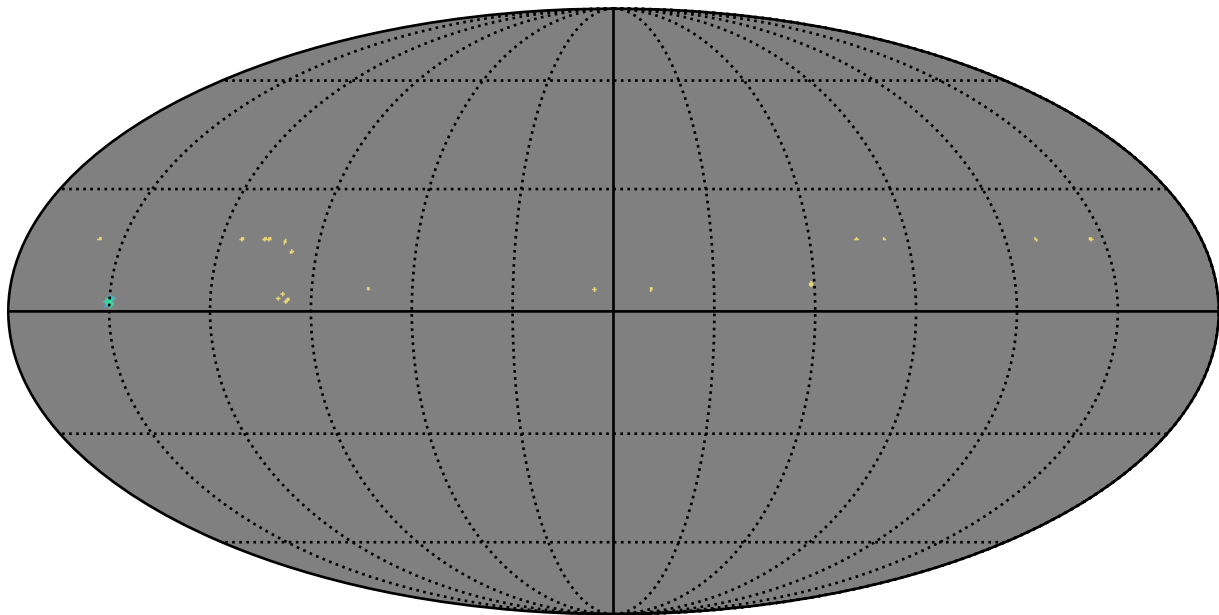
mw_roll_bulge_v3.3_10yrs y band: AGN_TimeLag_5_days
