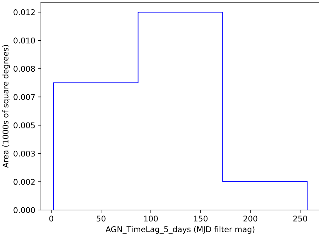
mw_roll_bulge_v3.3_10yrs y band: AGN_TimeLag_5_days
