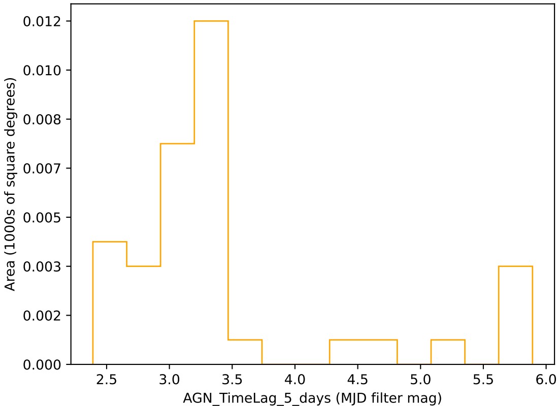
mw_roll_bulge_v3.3_10yrs r band: AGN_TimeLag_5_days
