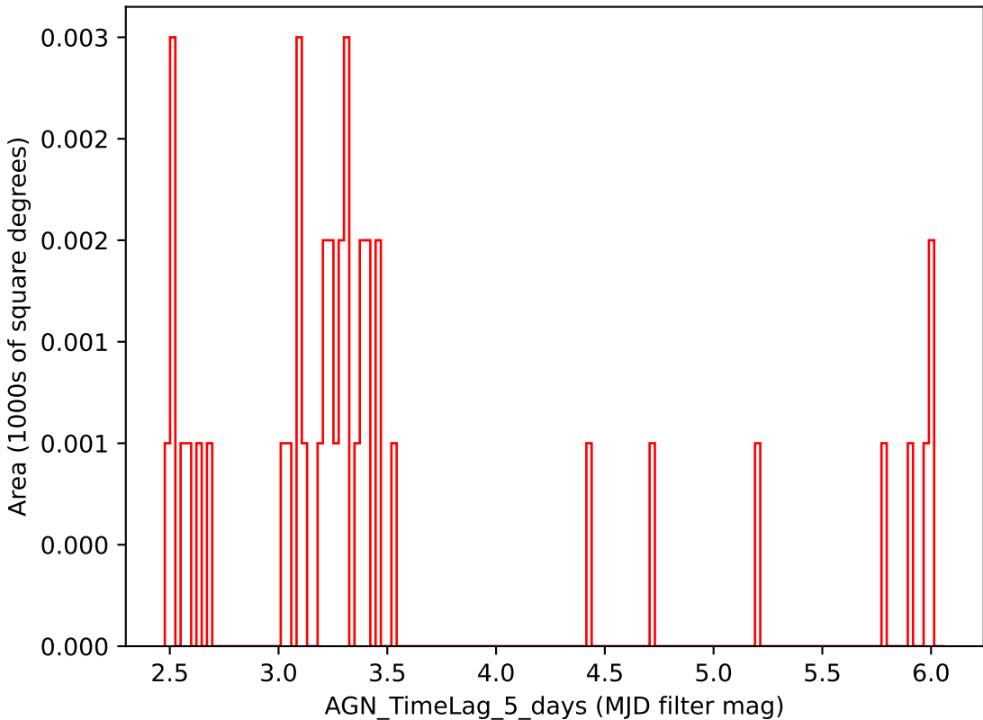
mw_roll_bulge_v3.3_10yrs i band: AGN_TimeLag_5_days
