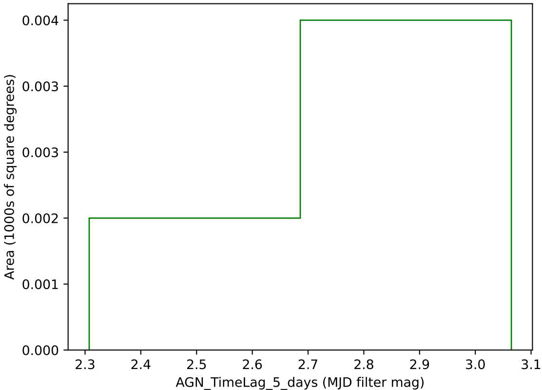
mw_roll_bulge_v3.3_10yrs g band: AGN_TimeLag_5_days
