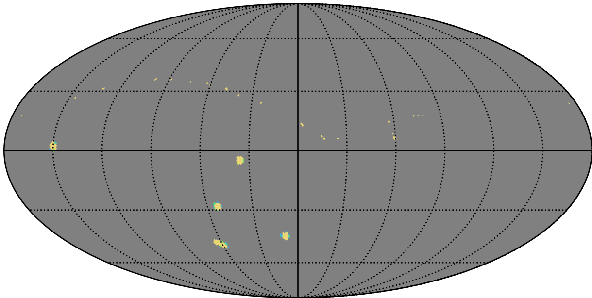
mw_roll_bulge_v3.3_10yrs all bands: AGN_TimeLag_5_days
