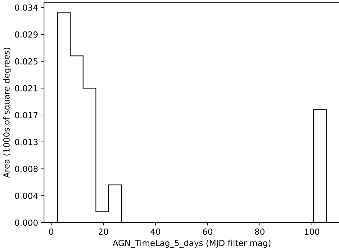
mw_roll_bulge_v3.3_10yrs all bands: AGN_TimeLag_5_days
