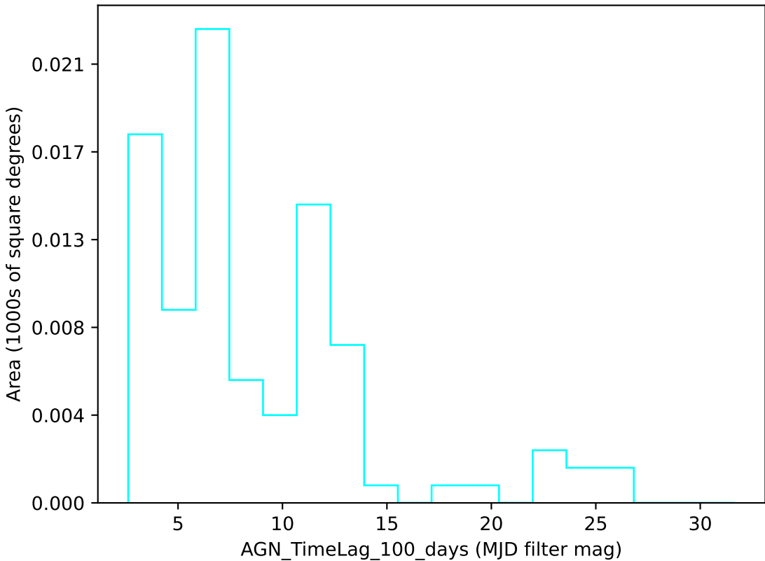
mw_roll_bulge_v3.3_10yrs u band: AGN_TimeLag_100_days
