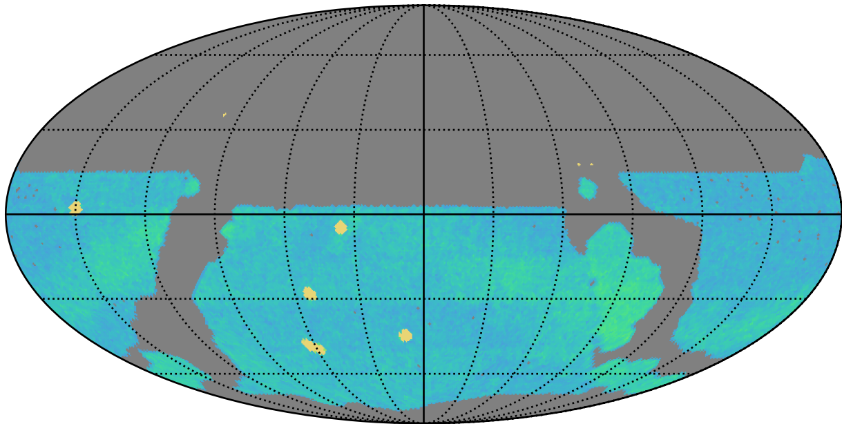
mw_roll_bulge_v3.3_10yrs r band: AGN_TimeLag_100_days
