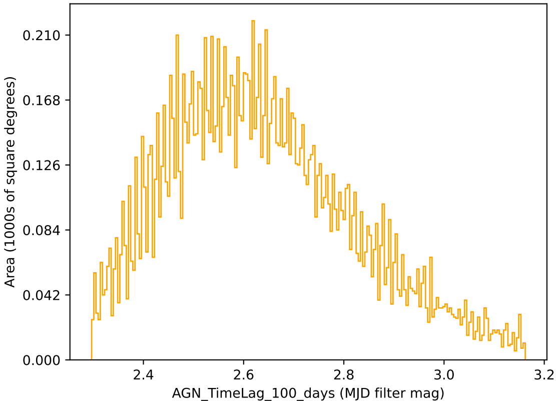
mw_roll_bulge_v3.3_10yrs r band: AGN_TimeLag_100_days
