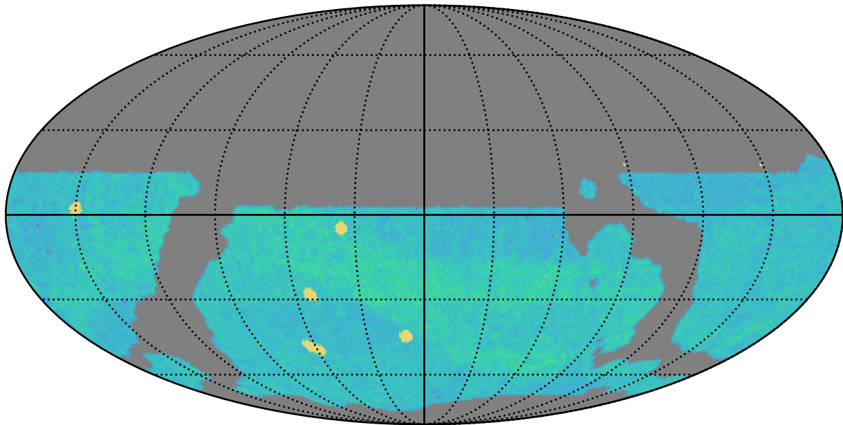
mw_roll_bulge_v3.3_10yrs i band: AGN_TimeLag_100_days
