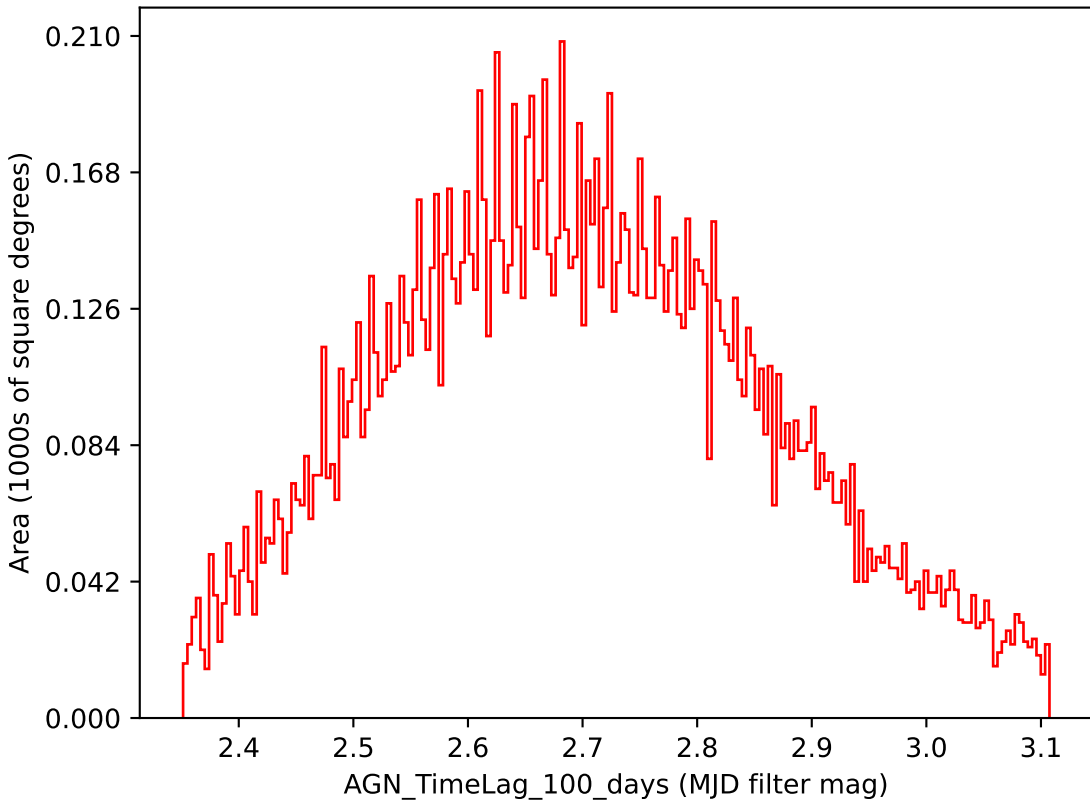
mw_roll_bulge_v3.3_10yrs i band: AGN_TimeLag_100_days
