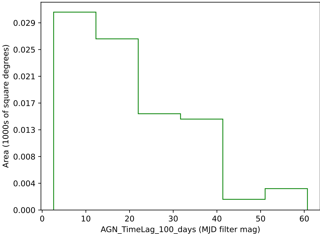
mw_roll_bulge_v3.3_10yrs g band: AGN_TimeLag_100_days
