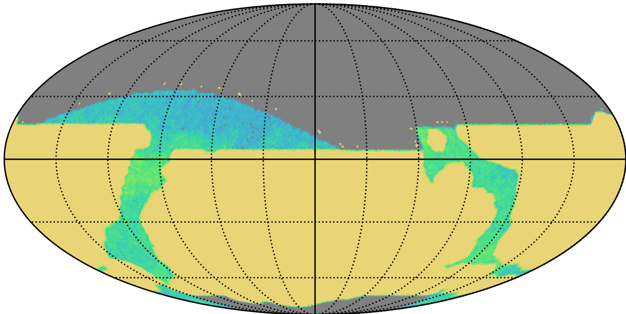
mw_roll_bulge_v3.3_10yrs all bands: AGN_TimeLag_100_days
