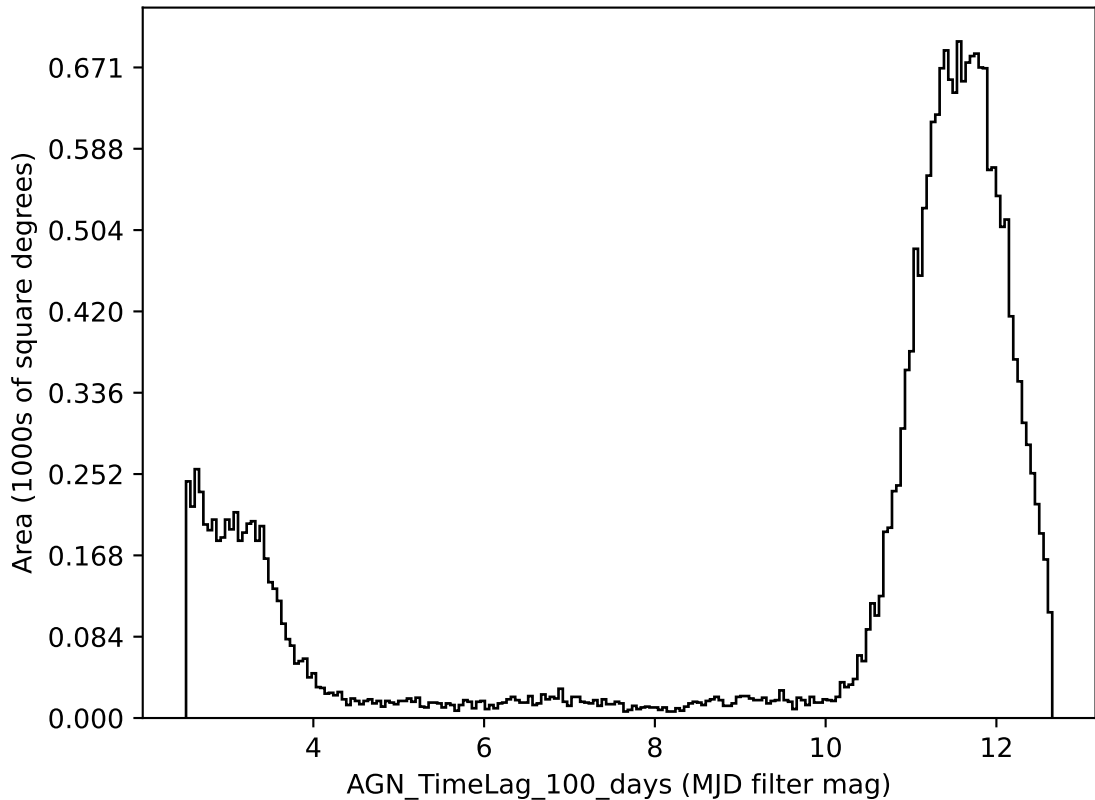
mw_roll_bulge_v3.3_10yrs all bands: AGN_TimeLag_100_days
