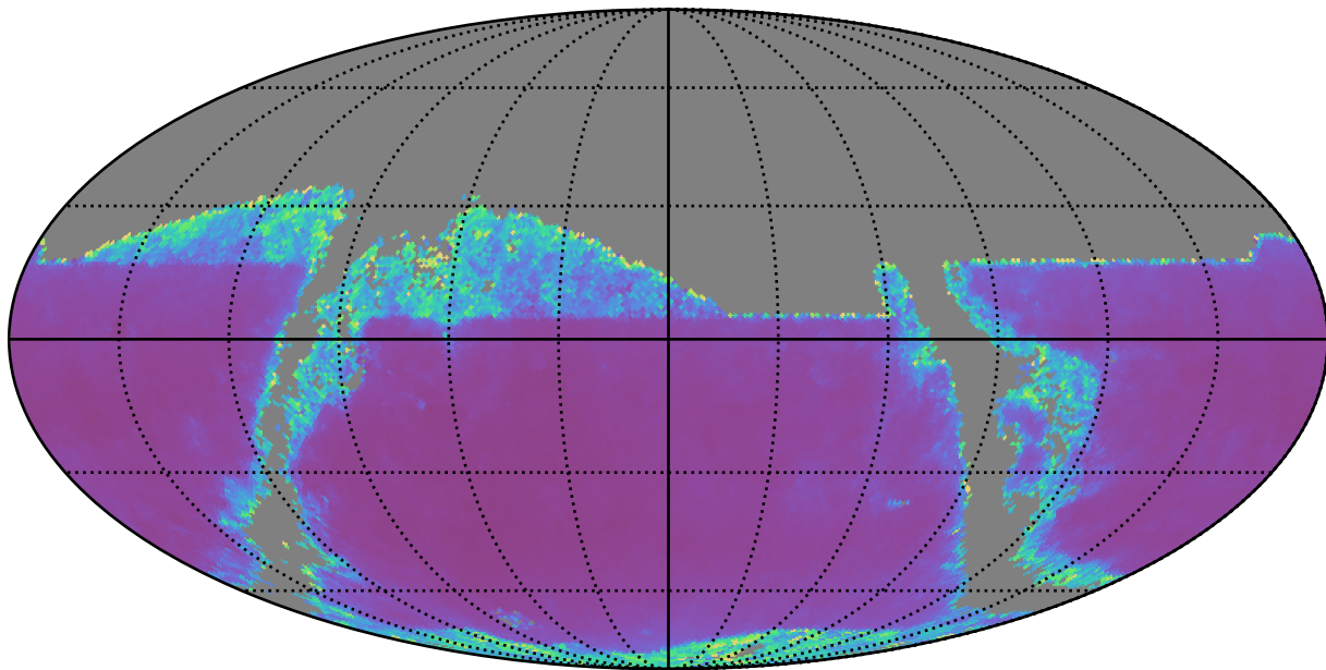
mw_roll_bulge_v3.3_10yrs z band: AGN SF_uncert
