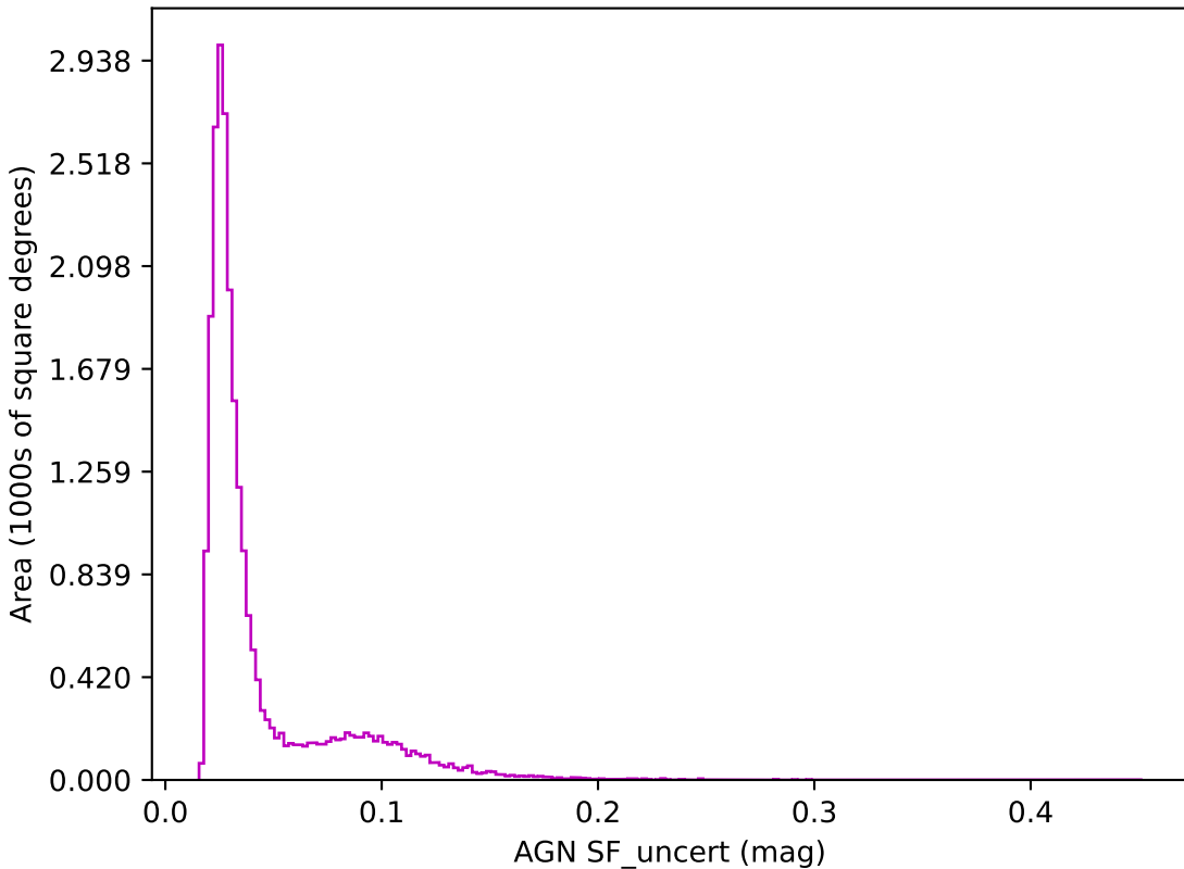
mw_roll_bulge_v3.3_10yrs z band: AGN SF_uncert
