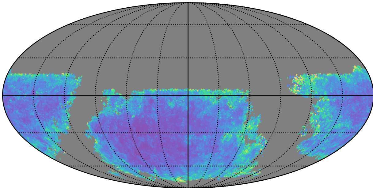
mw_roll_bulge_v3.3_10yrs u band: AGN SF_uncert
