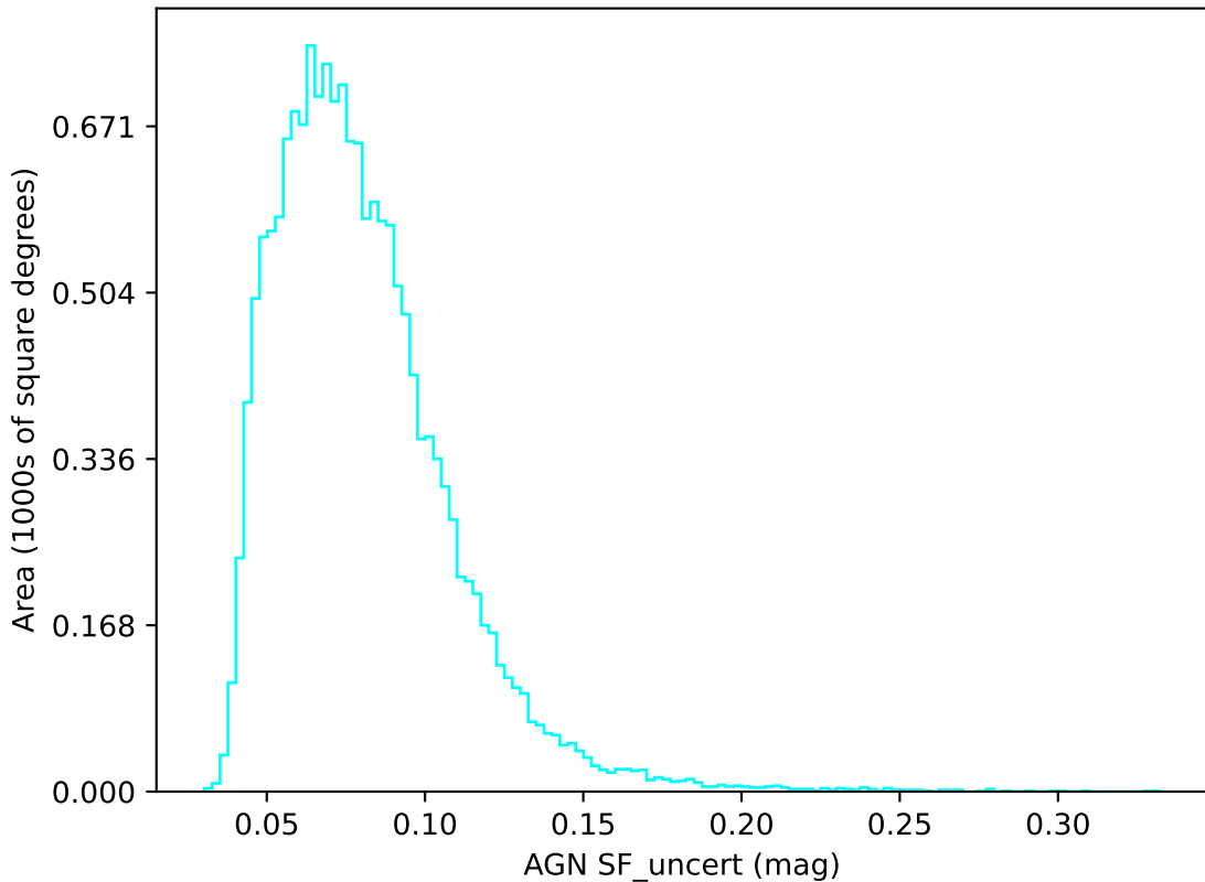
mw_roll_bulge_v3.3_10yrs u band: AGN SF_uncert
