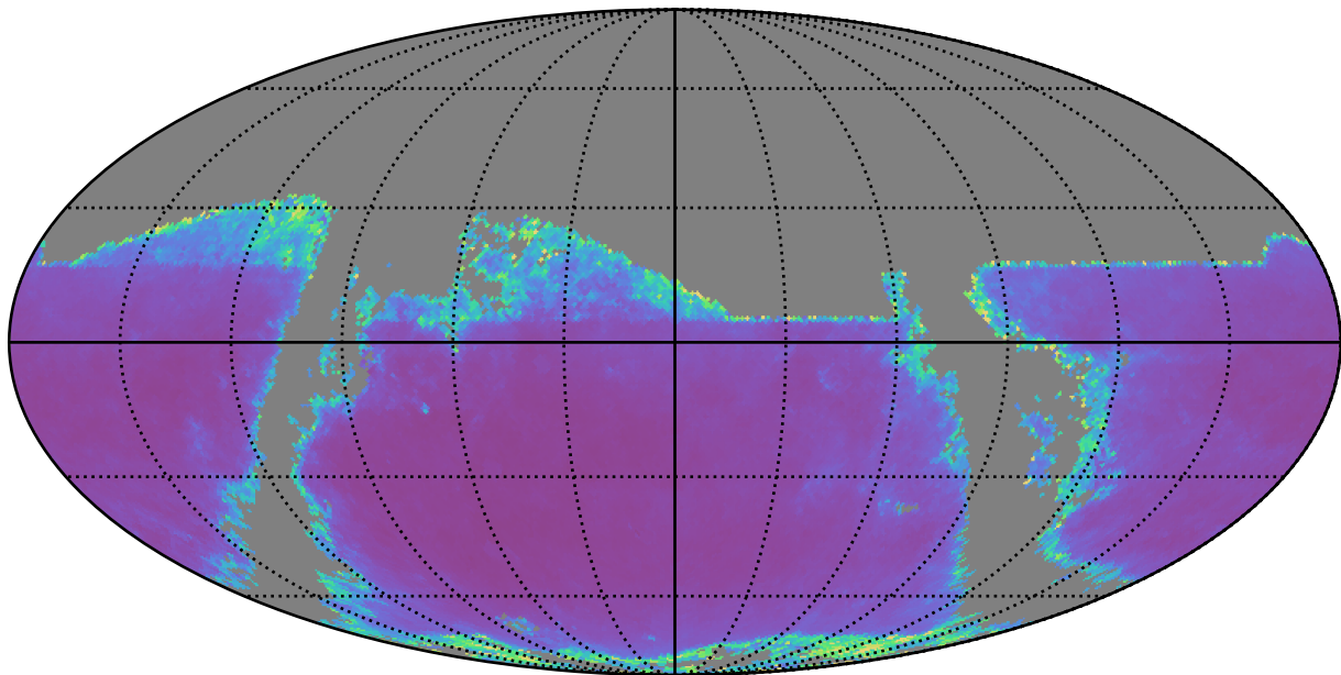
mw_roll_bulge_v3.3_10yrs r band: AGN SF_uncert
